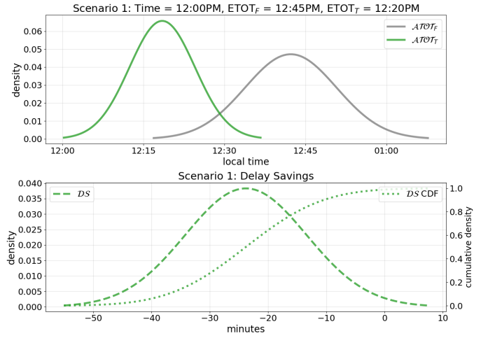
Fig. 8. Top: Scenario 1 \text{ATOT}_F and \text{ATOT}_T represent when we think the flight will take off on the filed and TOS alternative route, respectively. Bottom: Scenario 1 delay savings \mathcal{DS} and associated CDF
